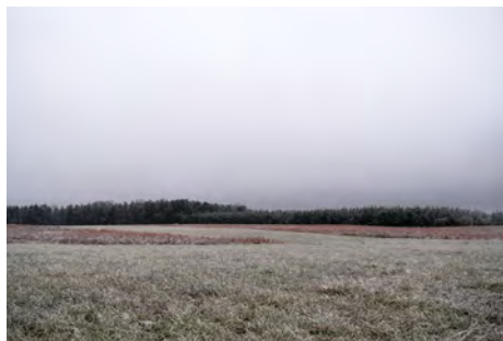
Stratus
